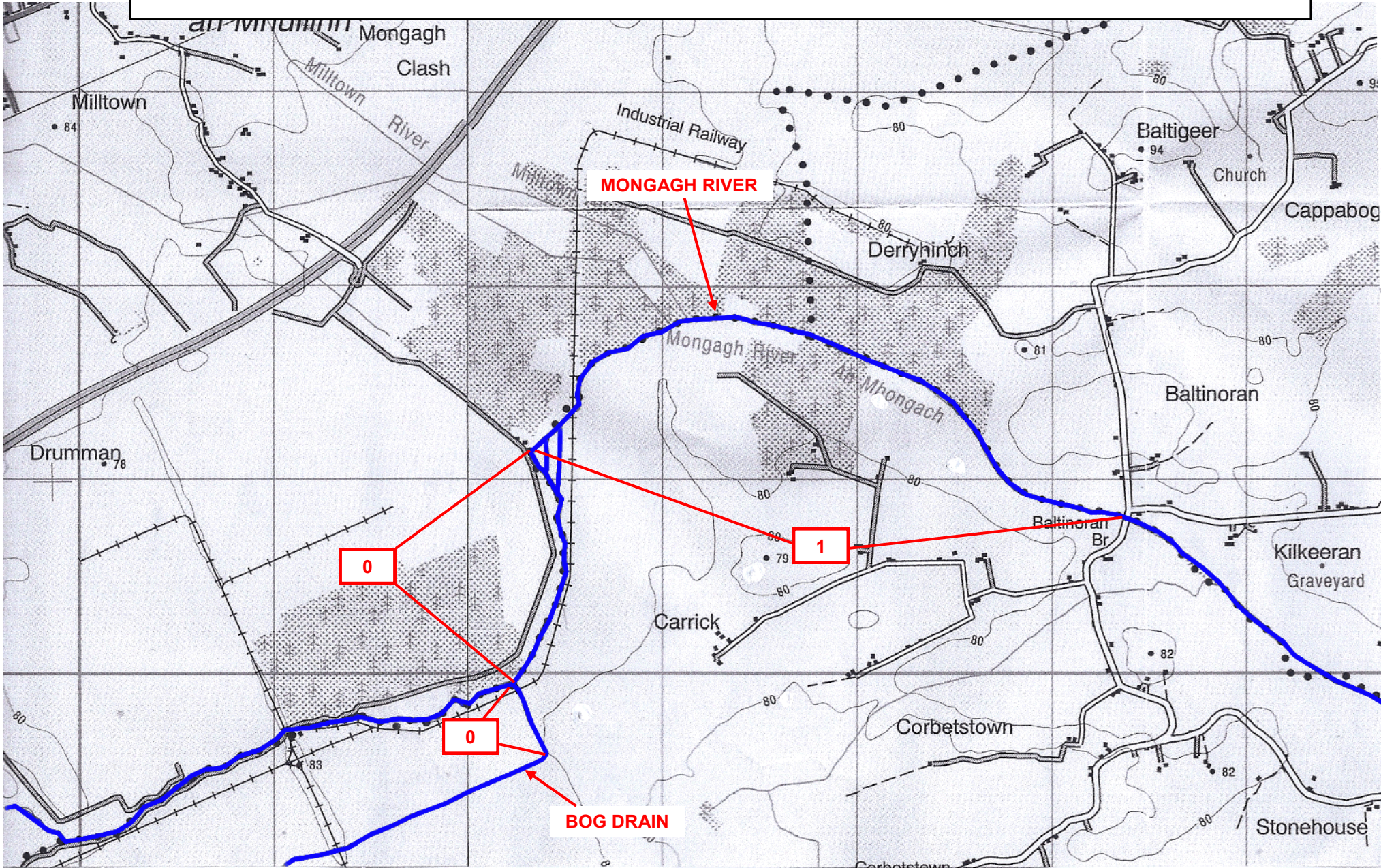
FIGURE 5.19 SALMONOID NURSERY HABITAT SECTIONS MONGAGH RIVER AND TRIBUTARY Rated on a scale of 0=None 2=Poor 4=Fair 6=Good 8=V.Good 10=Excellent
